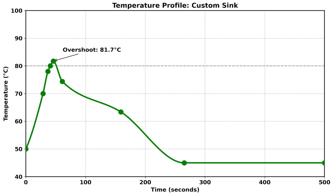
Fig 9 : Plot results for heating element with perforated heat sink temperature change w.r.t. time
