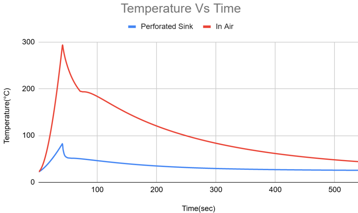
Fig 8: Ansys reading for heating element with and without perforated heat sink under natural convection
