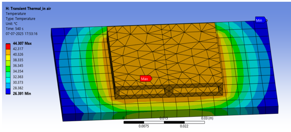
Fig 6: ANSYS transient thermal simulations for heating element under natural convection without heat sink
