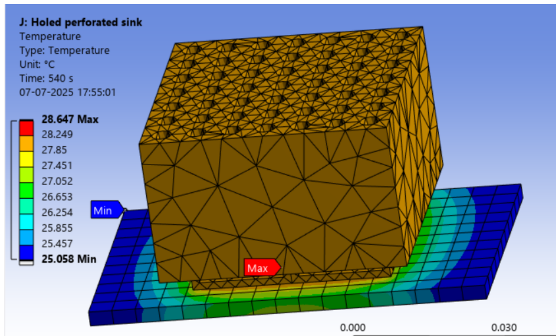
Fig 7: ANSYS transient thermal simulations for heating element mounted with perforated heat sink under natural convection
